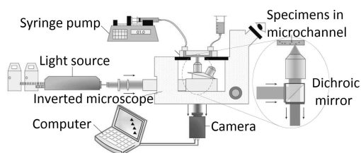
Figure 1: Schematic view of a micro-PIV setup using an inverted microscope. The illumination light is reflected by a dichroic mirror into a flowing microchannel being charged by a syringe pump. The reflected light passes through the dichroic mirror, recorded by a CCD or CMOS camera, and then digitally processed.
