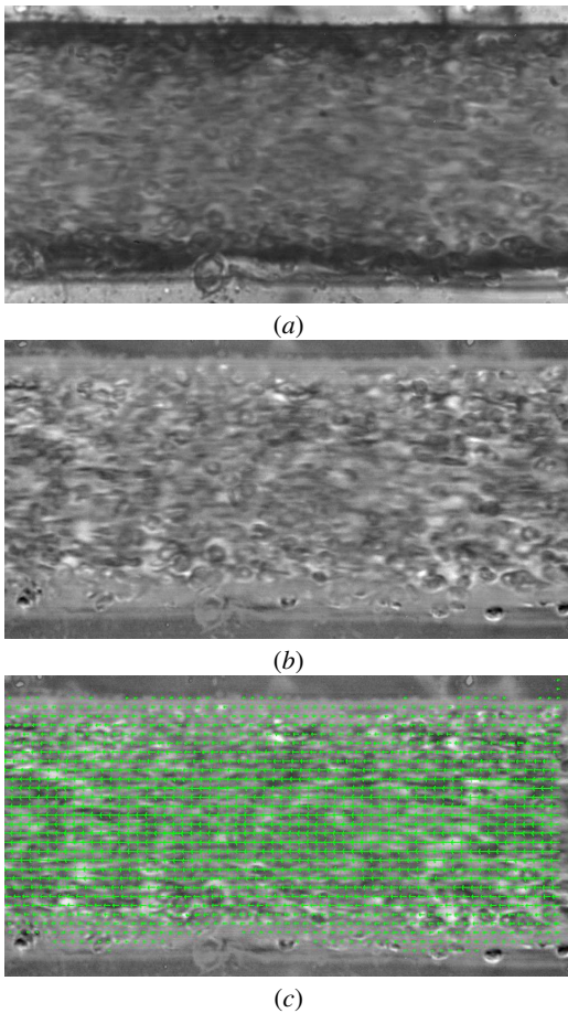
Figure 3: (a) Snapshot of 20% Hct RBCs treated with 0.00175% glutaraldehyde flowing through a 100 \times 100 \mu\text{m} straight channel at 100 nl/s captured using Y4 camera at 2000 frame per second. (b) Image enhancement of figure 3(a) using local sub notch averaging (c) Average velocity flow field over 2000 frames imposed on figure 3(b).
