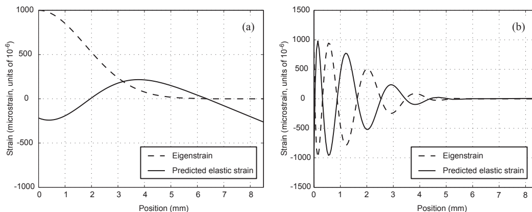
Figure 2. Eigenstrain and corresponding calculated elastic strain for Chebyshev polynomial ( T_k ) of degree (a) k=0 and (b) k=10
