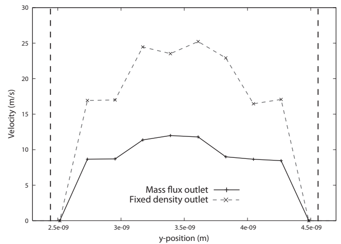
FIGURE 8. EFFECT OF OUTLET REPRESENTATION ON VELOCITY PROFILES INSIDE CNT; THE VERTICAL DASHED LINES INDICATE THE INTERNAL SURFACES OF THE CNT.
