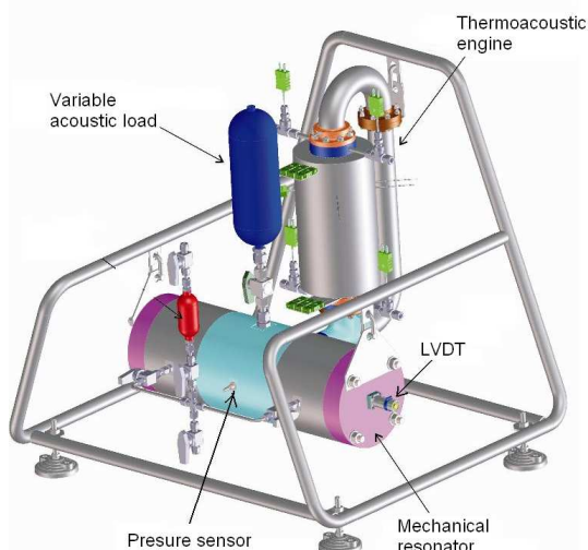
Figure 6. CAD-illustration of the thermoacoustic engine coupled to the mechanical resonator with instrumentation.
