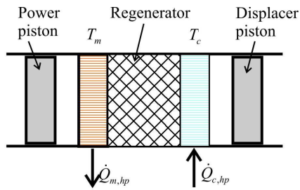
(a) Mechanical Stirling heat pump
