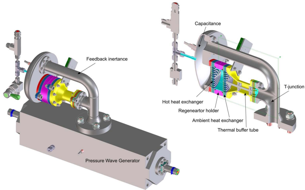
Figure 3. CAD model of the heat pump
