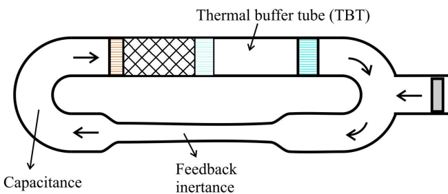
(b) Thermoacoustic Stirling heat pump
