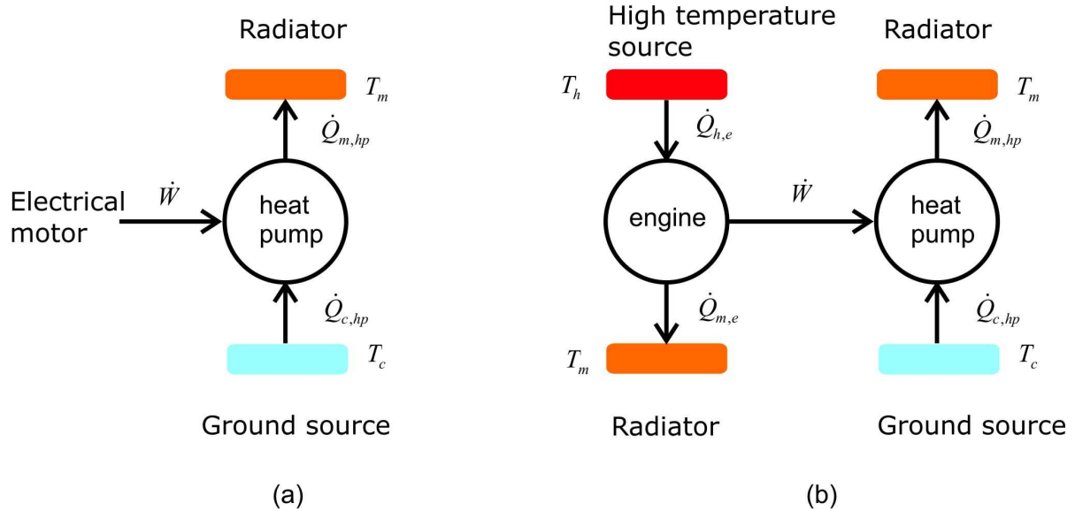
Figure 1. Illustration of a heat pump driven by an electrical motor (a) and a high temperature source such as a gas burner (b)
