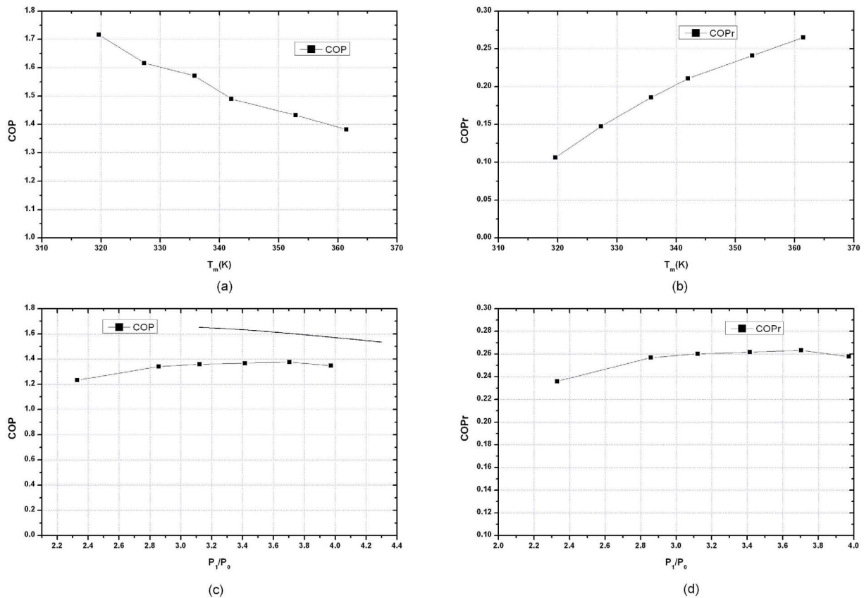
Figure 4. COP as function of hot temperature (a) and drive ratio (c). COP_r as a function of hot temperature (b) and drive ratio (d). These experiments were performed at a frequency of 98 Hz and an average pressure of 3.3 MPa. In (c) and (d) the inlet hot temperature of water is set to 80 °C.
